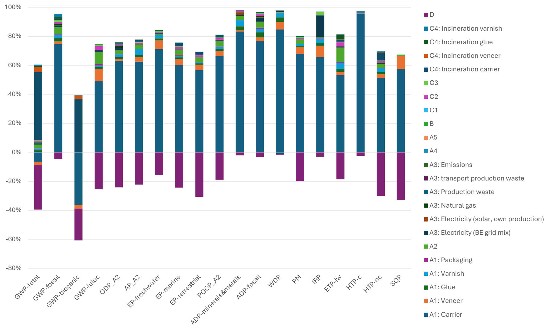
Figure 2 Major contributions to the environmental profile of Shinnoki panel
