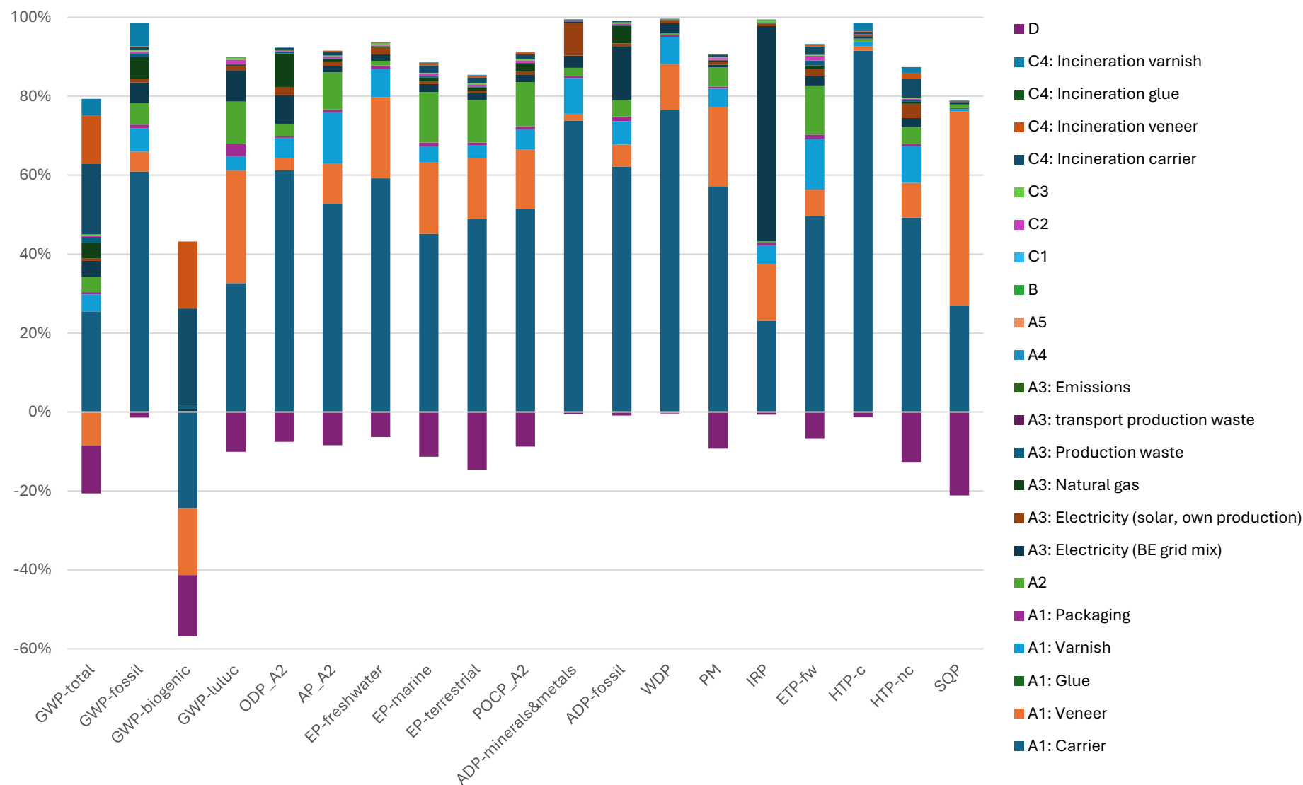
Figure 2 Major contributions to the environmental profile of Shinnoki laminate
