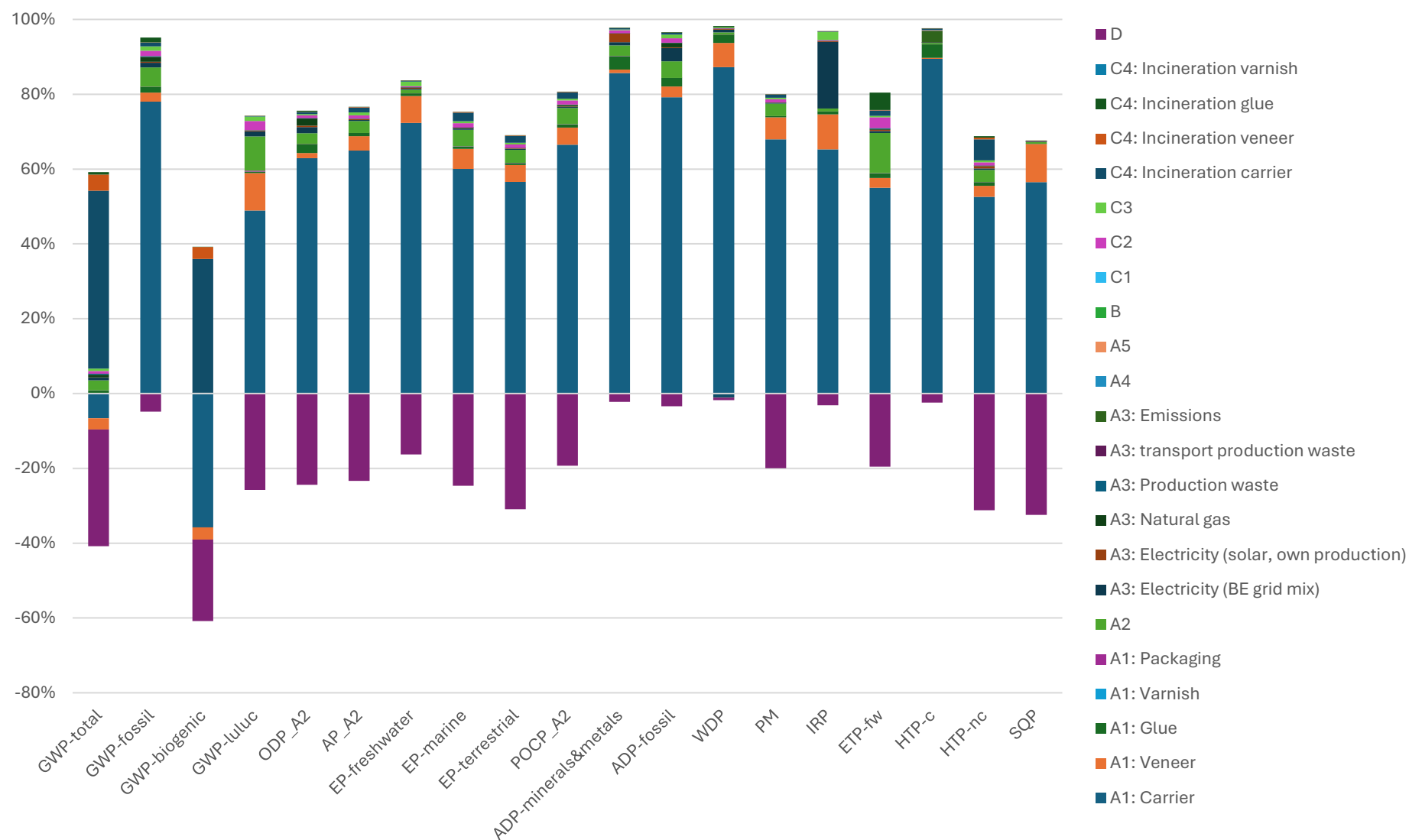
Figure 2 Major contributions to the environmental profile of veneered (0.6 mm) MDF
