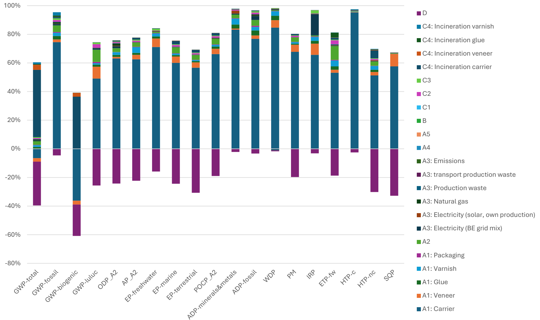
Figure 2 Major contributions to the environmental profile of veneered (0.6 mm) and finished MDF
