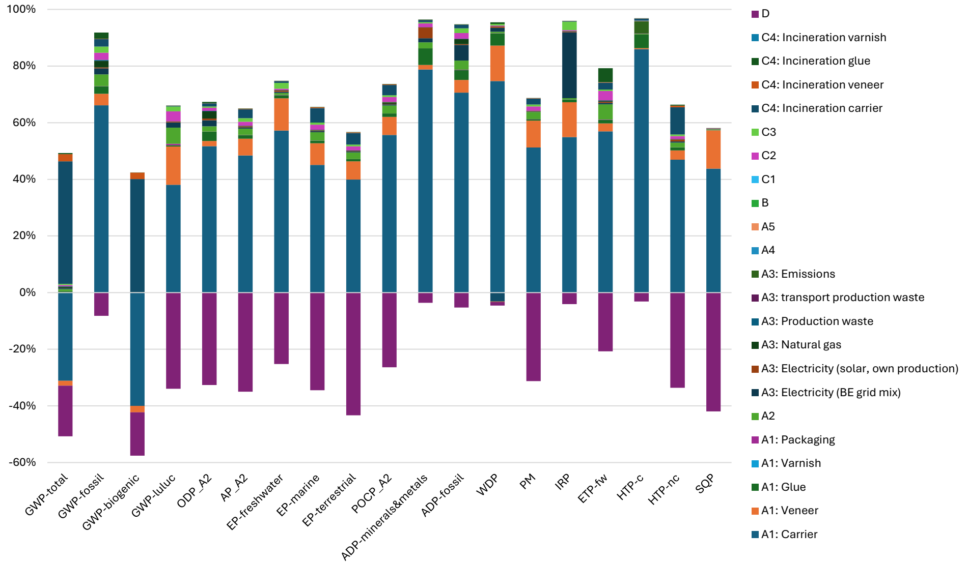
Figure 2 Major contributions to the environmental profile of veneered (0.6 mm) chipboard
