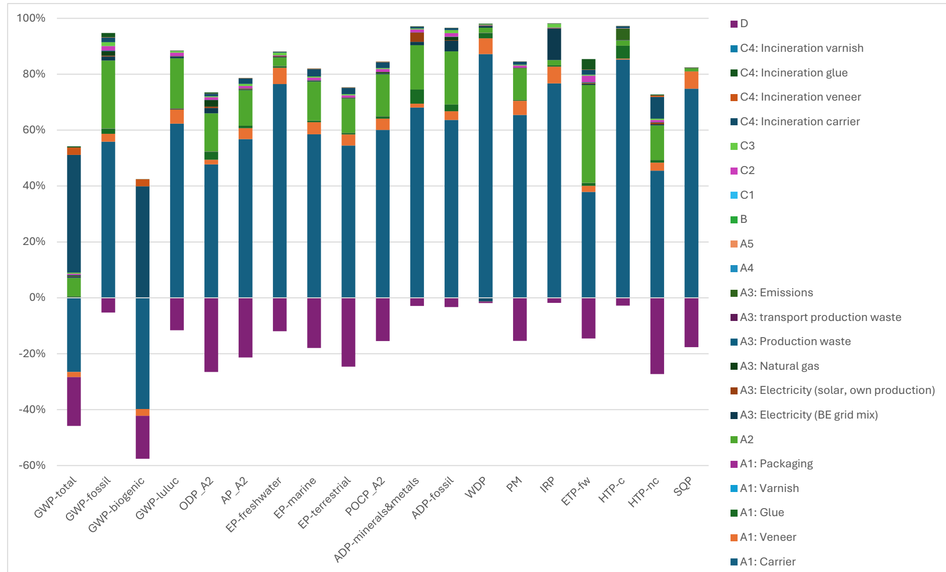
Figure 2 Major contributions to the environmental profile of veneered (0.6 mm) plywood
