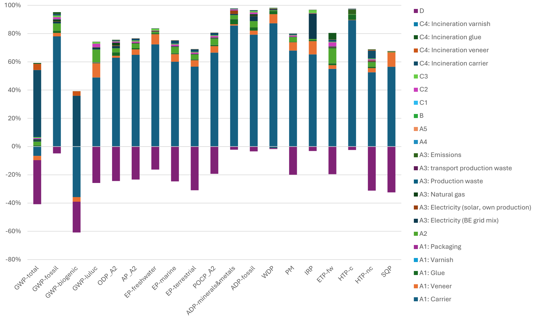
Figure 2 Major contributions to the environmental profile of Querkus panel (0,6 mm)
