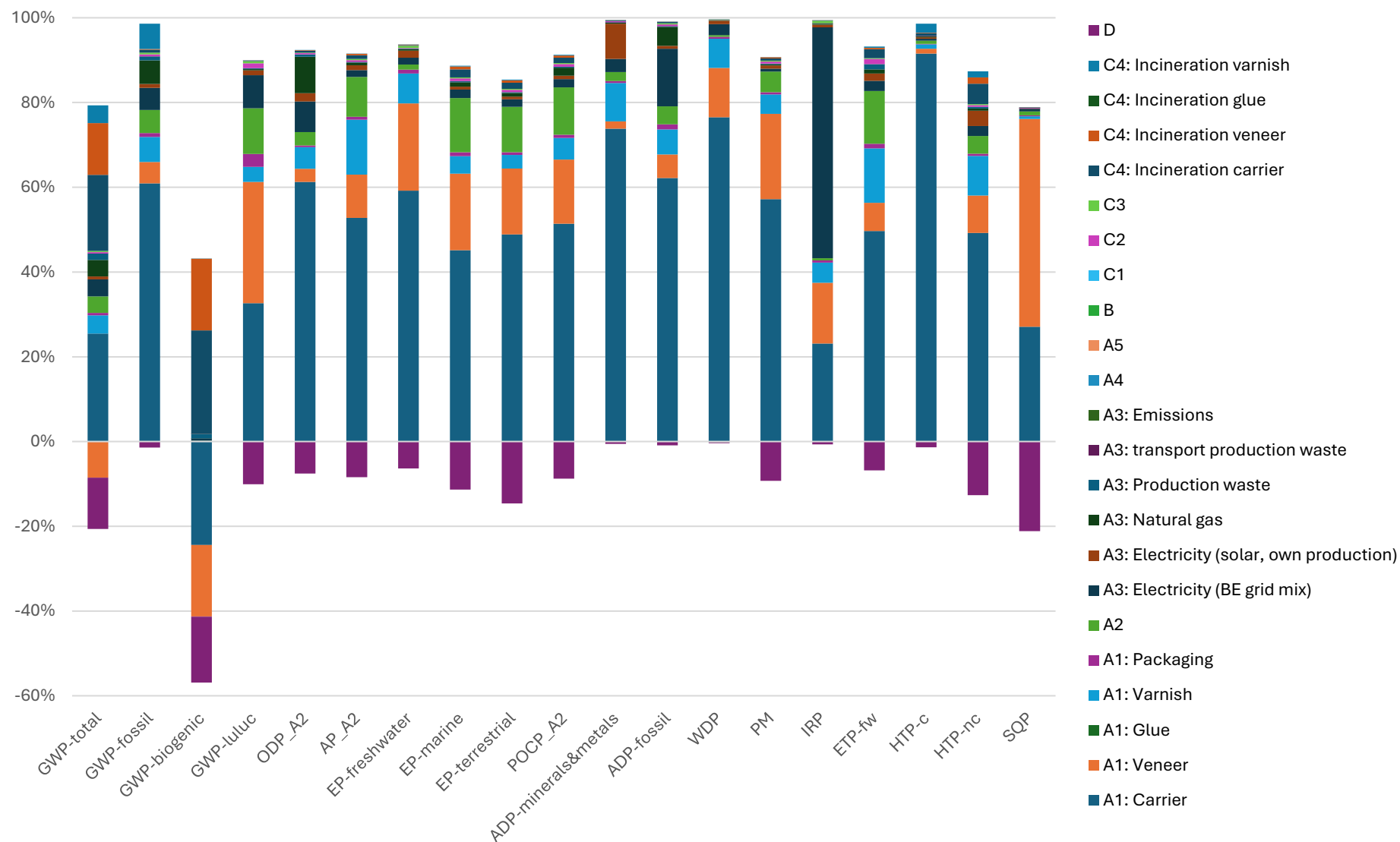
Figure 2 Major contributions to the environmental profile of Veneered (0,6 mm) and varnished laminate - Decolam
